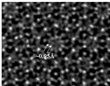
Fig.1 STEM image (processed) of a decagonal \text{Al}_{72}\text{Ni}_{20}\text{Co}_8 .
